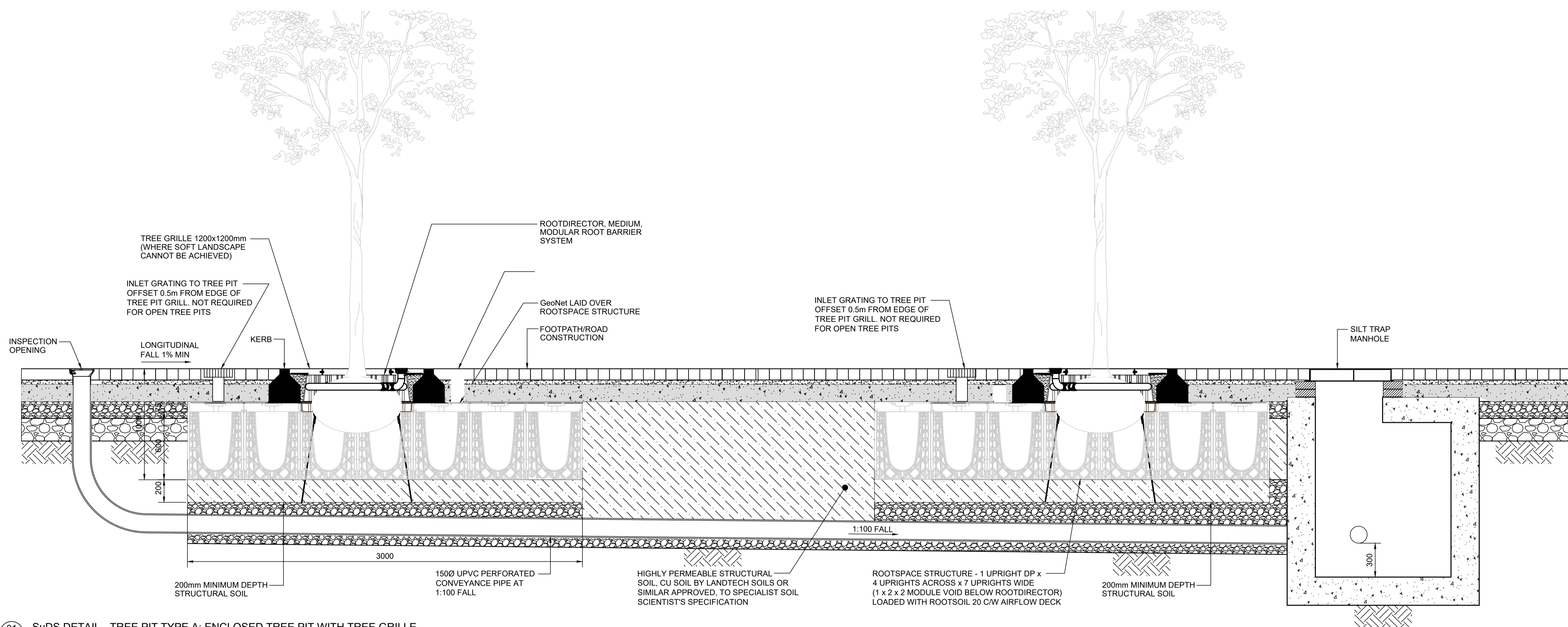
01 SuDS DETAIL - TREE PIT TYPE A: ENCLOSED TREE PIT WITH TREE GRILLE SCALE: 1:20@A1
