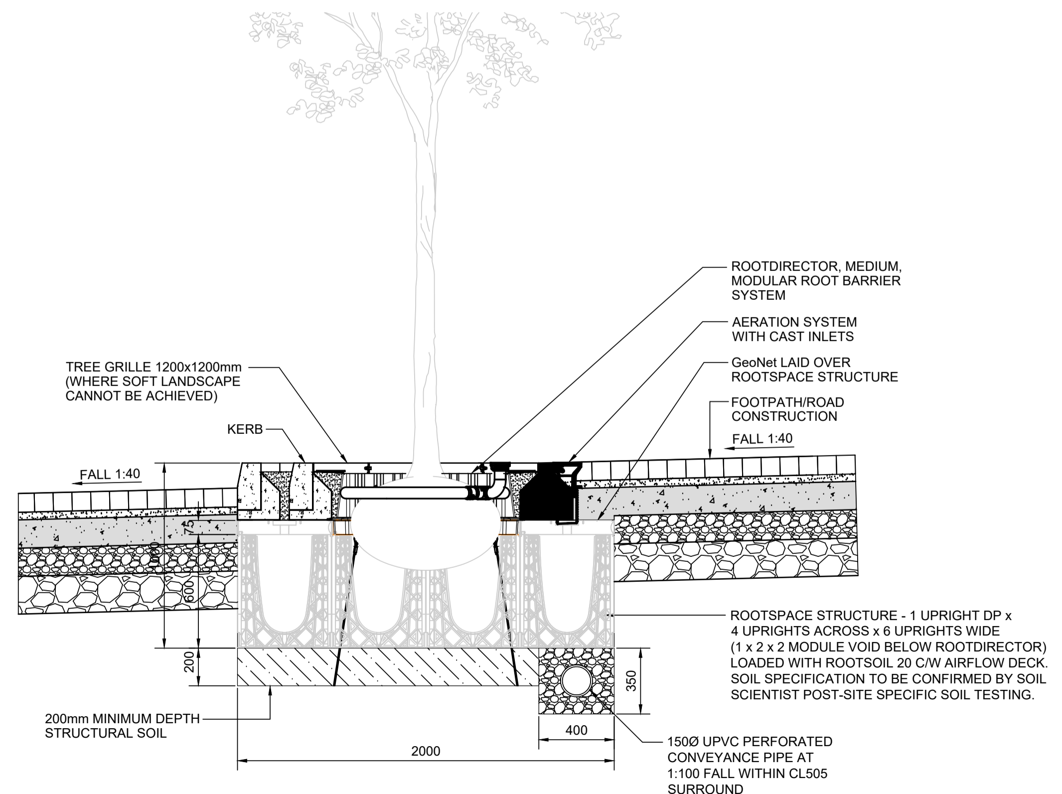
02 BR1: BIO-RETENTION TREE PIT SCALE: 1:20@A1
